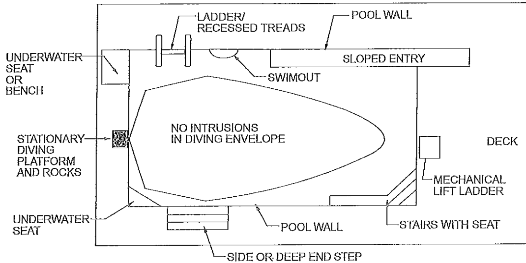
FIGURE 322.2 MINIMUM WATER DIVING ENVELOPE
